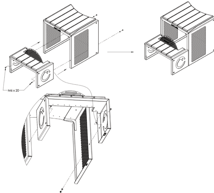
9.2 Figure. Connecting the stairs package's steps.
